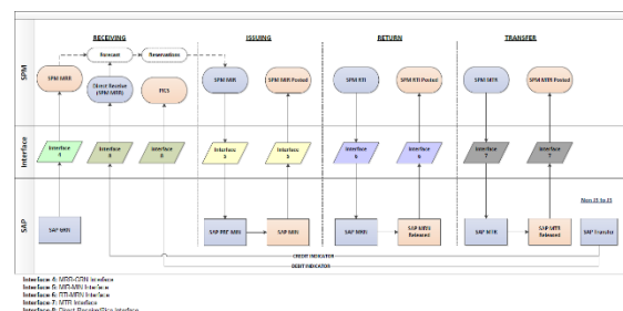
Interfaces between SmartPlant Materials (Site) and SAP
