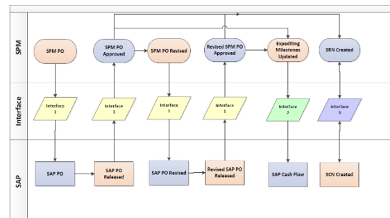
Interfaces between SmartPlant Materials (Material Supply Chain Management) and SAP
